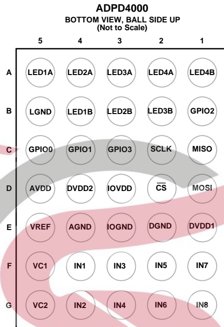
Figure 5. ADPD4000 Pin Configuration
