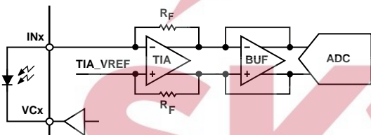
Figure 41. Signal Path for Digital Integration Mode
