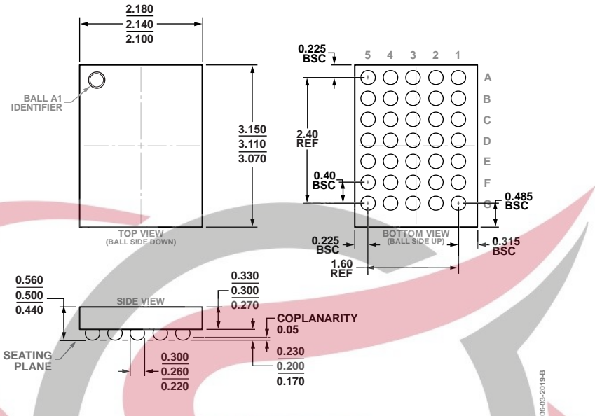
Figure 46. 35-Ball Wafer Level Chip Scale Package [WLCSP] (CB-35-2) Dimensions shown in millimeters
