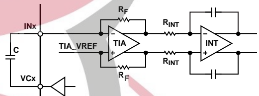
Figure 37. Modulate Stimulus for Capacitance Measurement
