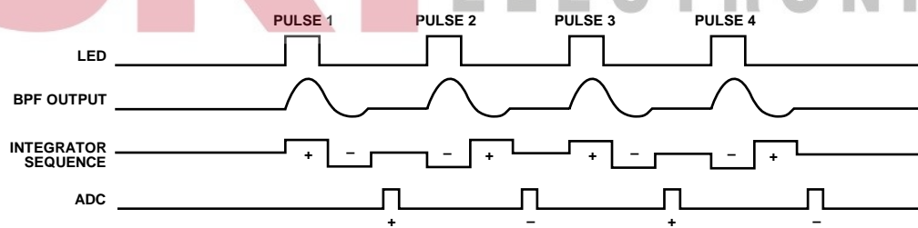
Figure 34. Diagram of Integrator Chopping Sequence
